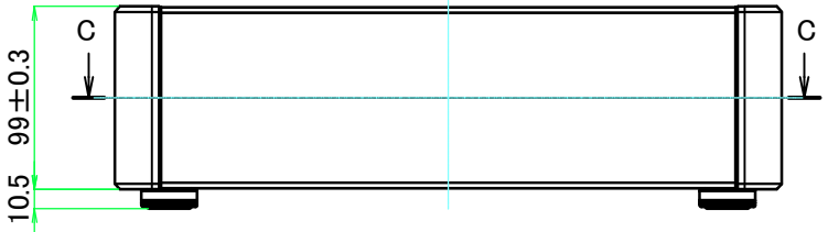
A view
